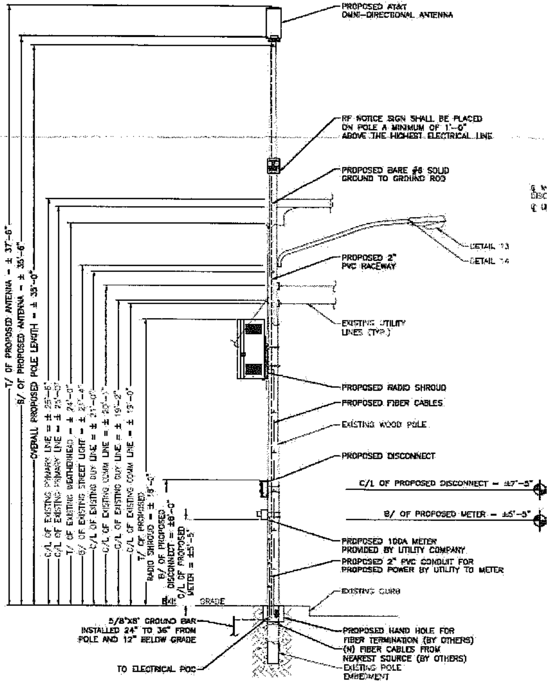
PROPOSED POLE ELEVATION
